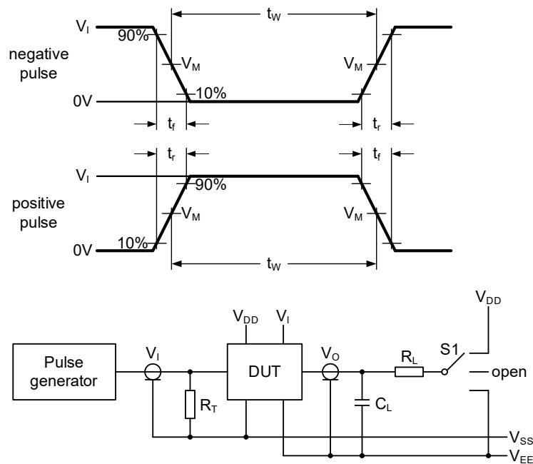
Figure 8-10 Test circuit for switching times
