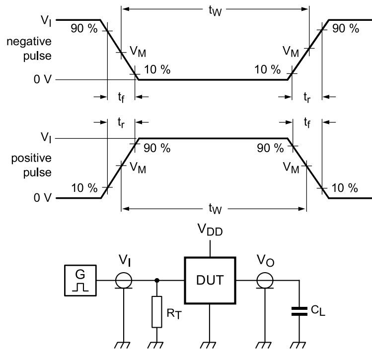
Figure 8-3 Test circuit for switching times
