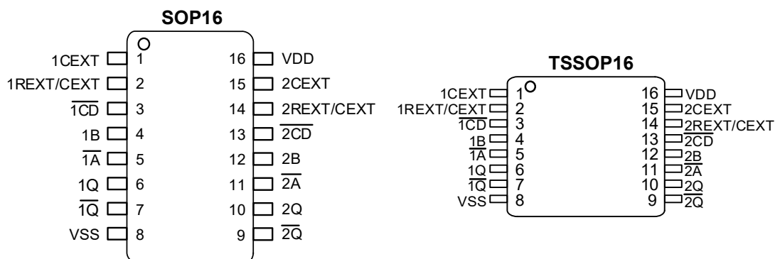
Figure 6-1 Pin configuration
