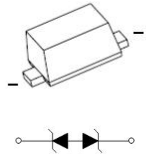
SOD-723
