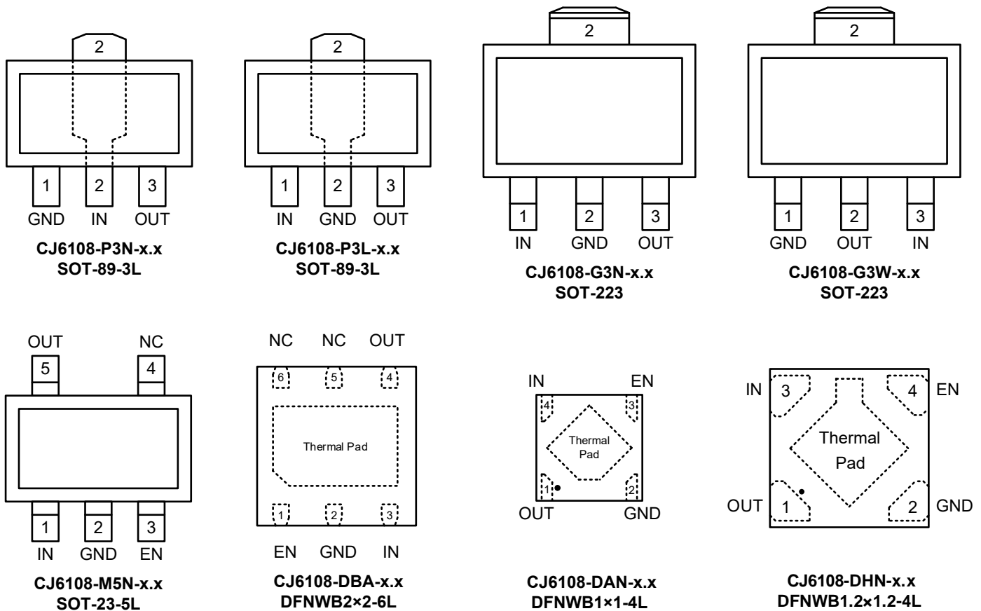
Figure 5-1. Package Top View (Not to Scale)
