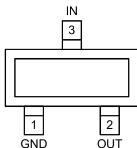
CJ6213-N3N-x.x SOT-23
