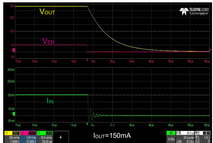
V_{OUT} = 3.3V , V_{IN} = 12V , Power Off
