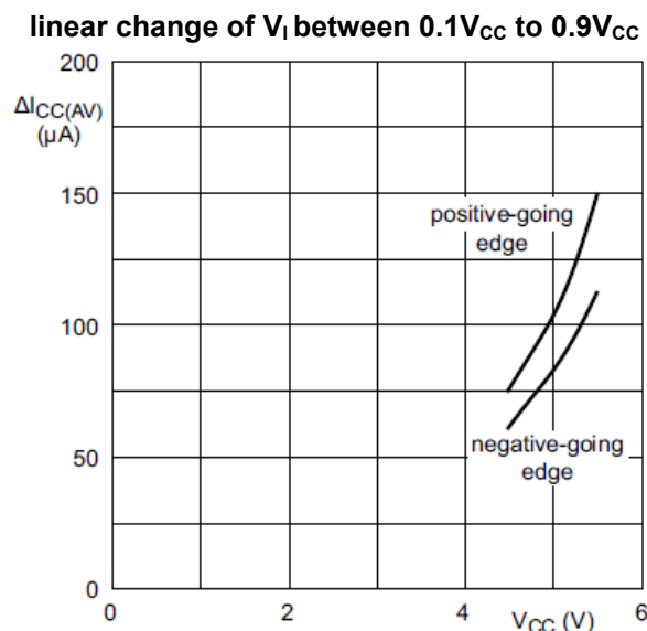
Figure 8-14 Average additional I_{CC} for CJ74AHCT1G14 Schmitt trigger devices;
