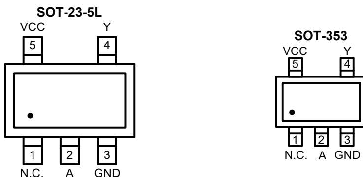
Figure 6-1 Pin configuration
