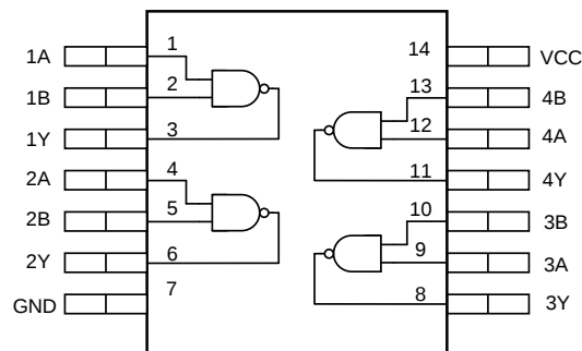
Device Functional Pinout
