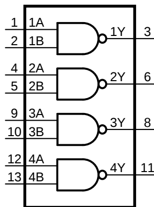
Figure 8-1 Logic symbol
