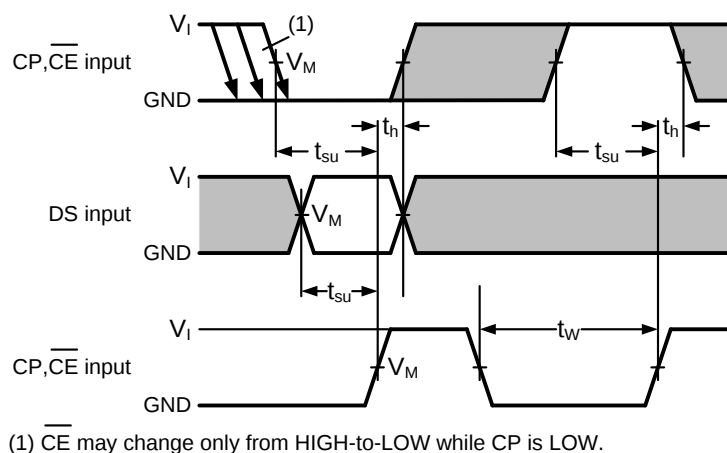
Figure 8-9 The set-up and hold times from the serial data input (DS) to the clock (CP) and clock enable ( \overline{\text{CE}} ) inputs, from the clock enable input ( \overline{\text{CE}} ) to the clock input (CP) and from the clock input (CP) to the clock enable input ( \overline{\text{CE}} )
