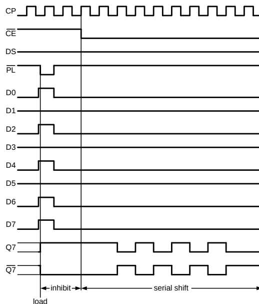
Figure 8-4 Timing diagram
