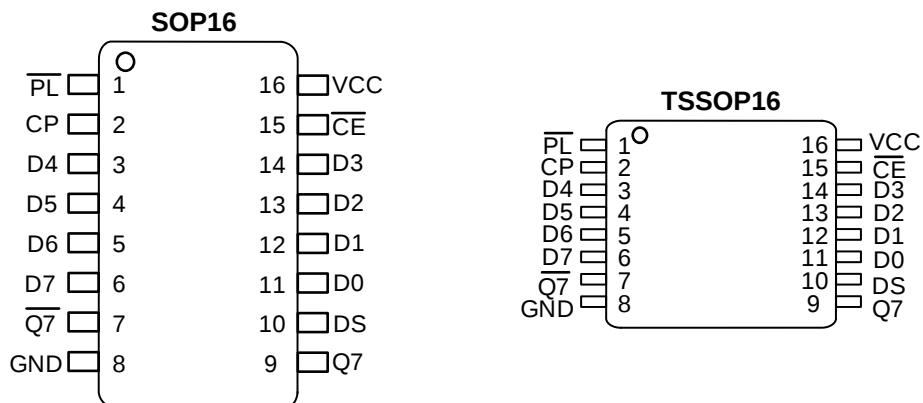
Figure 6-1 Pin Configuration
