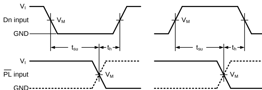
Figure 8-10 The set-up and hold times from the data inputs (Dn) to the parallel load input ( \overline{\text{PL}} )
