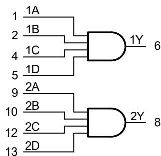
Figure 8-1 Logic symbol
