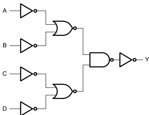
Figure 8-3 Logic diagram
