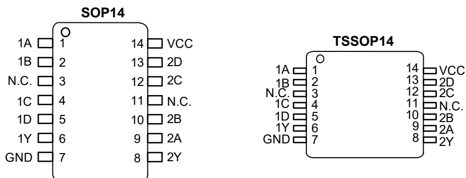
Figure 6-1 Pin configuration
