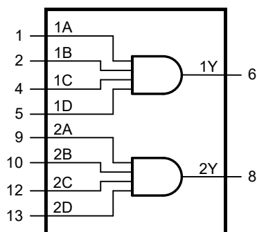
Figure 8-4 Functional diagram
