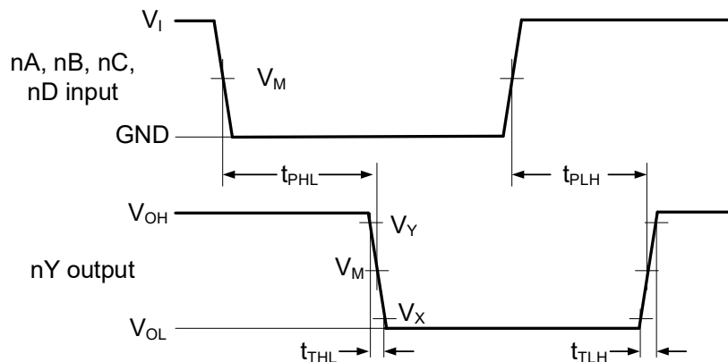
Figure 8-6 Waveforms showing the input (nA, nB, nC, nD) to output (nY) propagation delays and the output transition times
