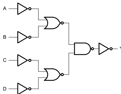
Logic diagram
