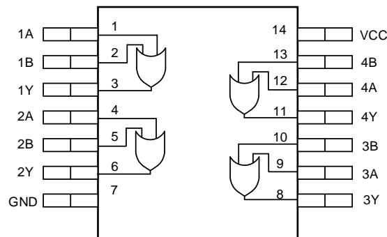
Functional pinout
