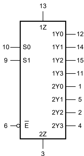
Figure 8-1 Logic symbol
