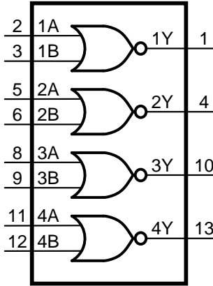
Figure 8-1 Logic symbol
