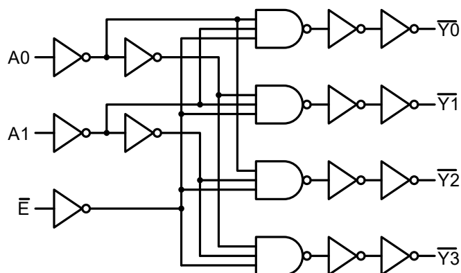
Figure 7-4 Logic diagram (one decoder/demultiplexer)
