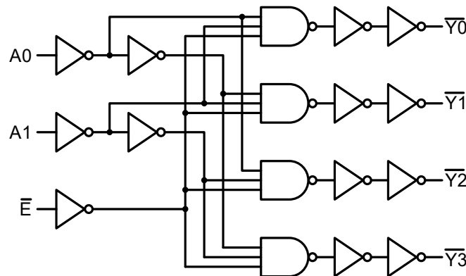
Logic diagram
