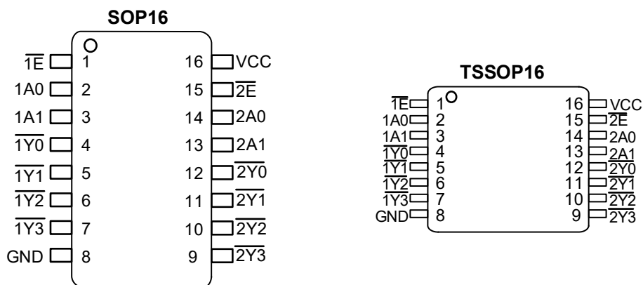
Figure 5-1 Pin configuration
