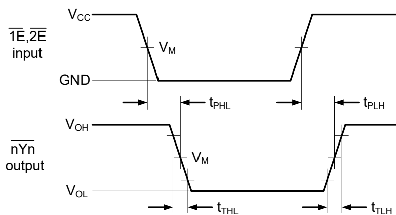
Figure 7-7 Propagation delay enable input (nE) to output (nYn) and transition time output (nYn)
