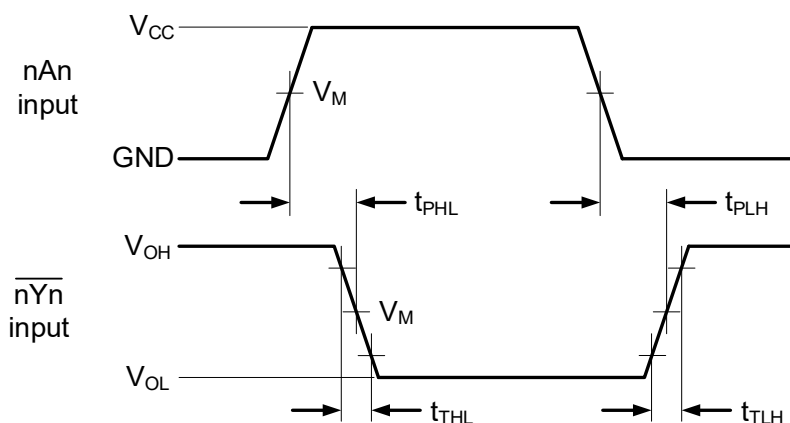
Figure 7-6 Propagation delay input (nAn) to output (nYn) and transition time output (nYn)
