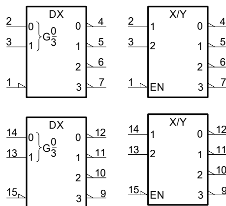
Figure 7-2 IEC logic symbol
