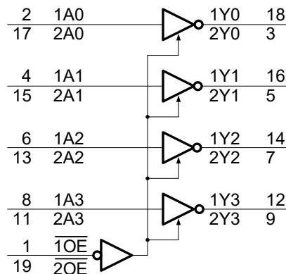
Logic symbol
