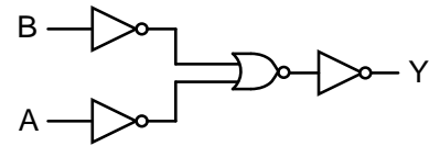
Figure 8-3 Logic diagram
