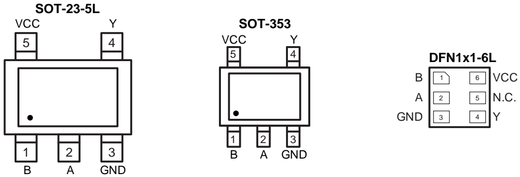
Figure 6-1 Pin configuration
