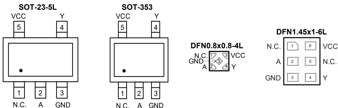
Figure 6-1 Pin configuration
