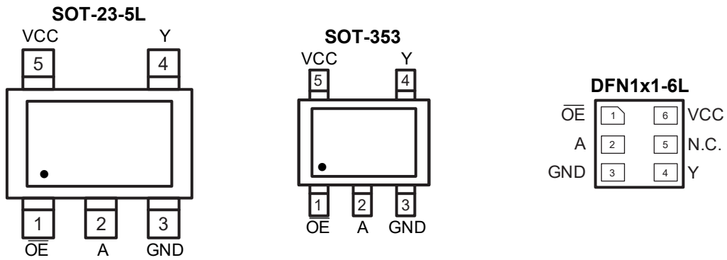
Figure 6-1 Pin configuration
