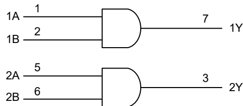
Functional diagram
