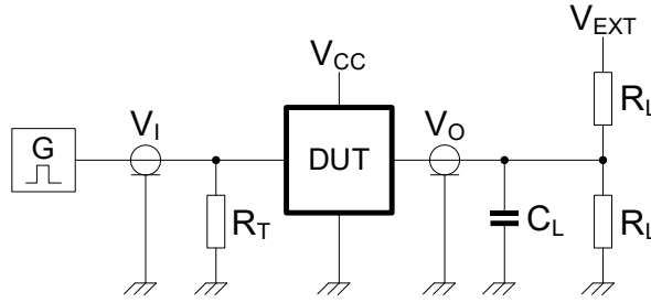
Figure 8-4 Test circuit for measuring switching times
