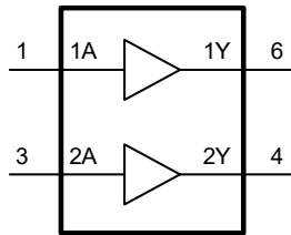
Figure 8-1 Logic symbol
