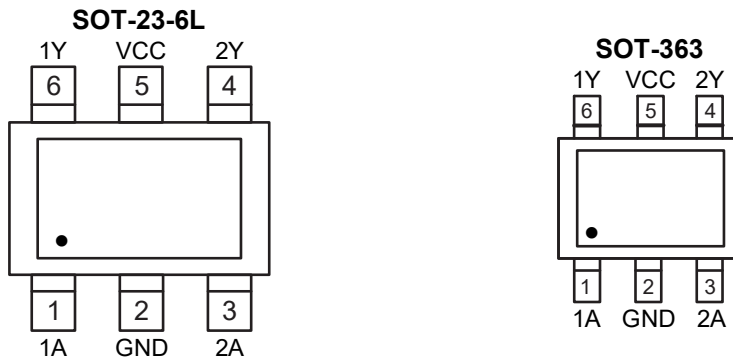
Figure 6-1 Pin configuration
