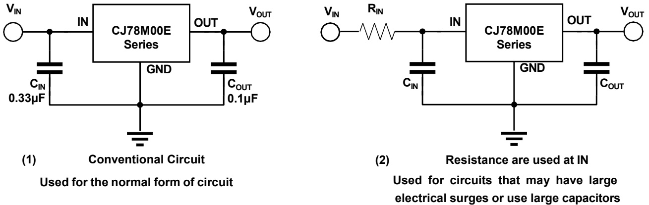
Figure 8-3. Fixed Output Regulator
