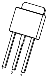
Figure 5-1. CJ78M00E Series Packages Top View
