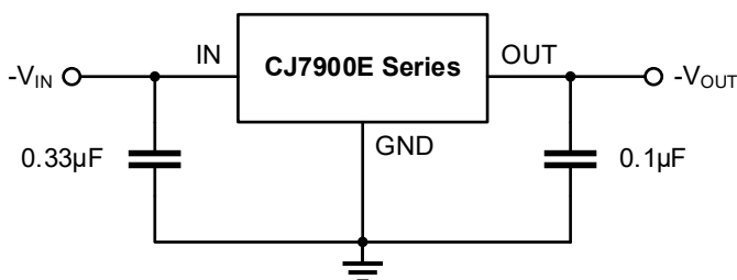
Figure 9-3. Conventional Circuit
