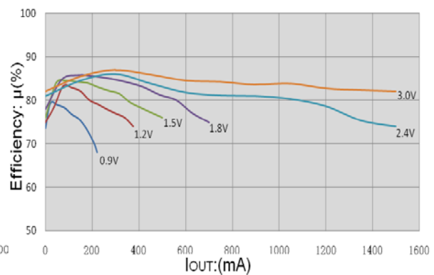
b、Efficiency \mu (%) vs. I_{OUT} :
