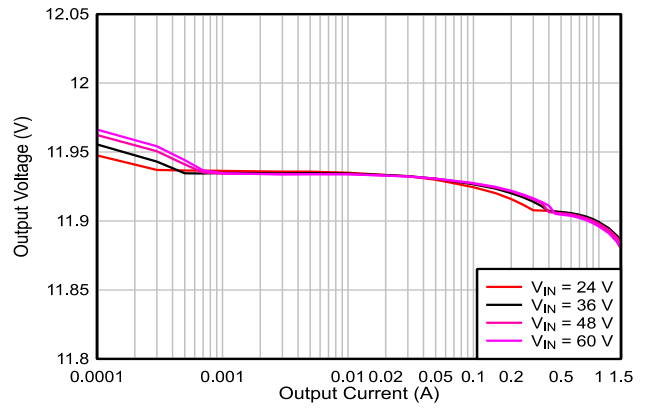
Load Regulation ( V_{OUT} = 12V , F_{SW} = 240KHz )
