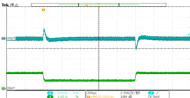
Load Transient (V_{OUT} = 12V, L=47\mu H, I_{OUT} = 0.75A \text{ to } 1.5A, 2.5A/\mu s \text{ slew rate})
