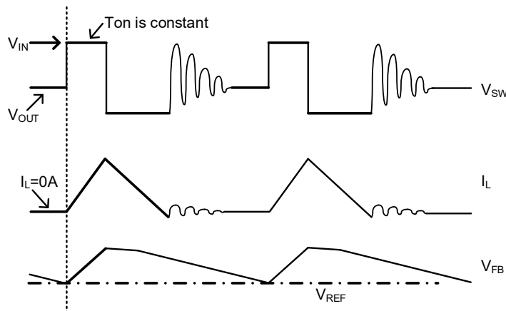
Figure 8-3 Light-Load Operation
