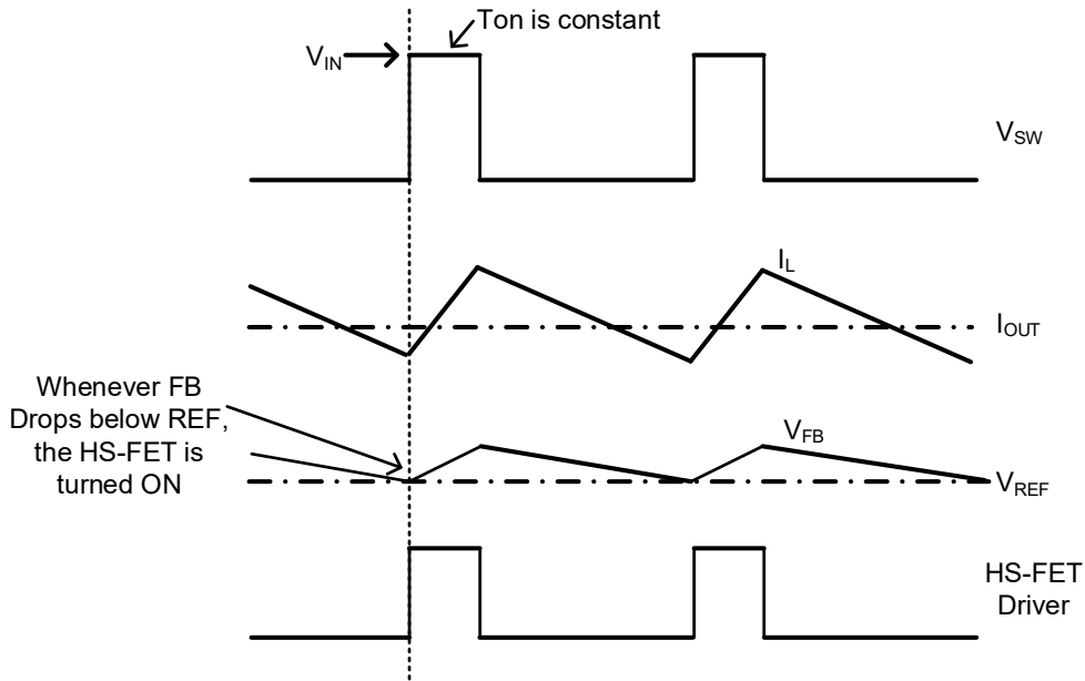
Figure 8-2 Heavy-Load Operation
