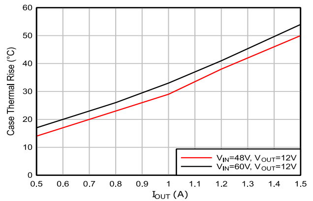
Thermal Rise ( V_{OUT} = 12V , F_{SW} = 240KHz , no air flow)
