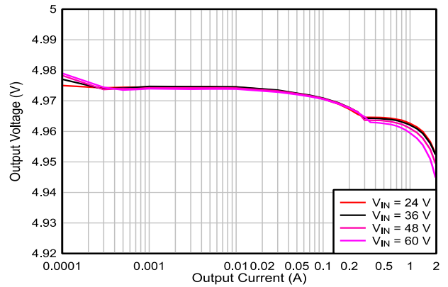
Load Regulation ( V_{OUT} = 5V , F_{SW} = 240KHz )
