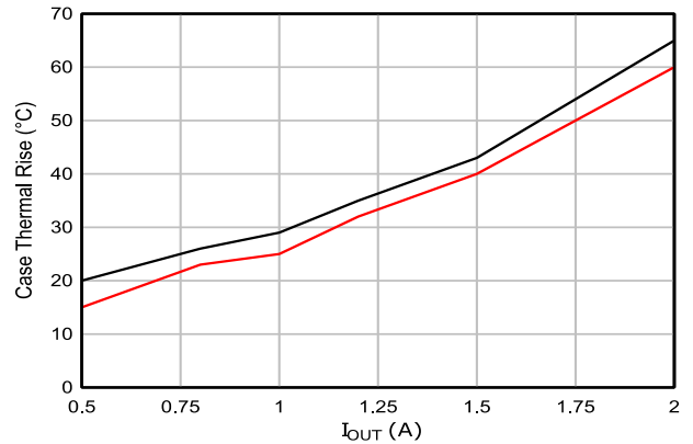
Thermal Rise ( V_{OUT} = 5V , F_{SW} = 240KHz , no air flow)
