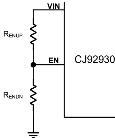
Figure 8-4 EN divider for adjustable UVLO
