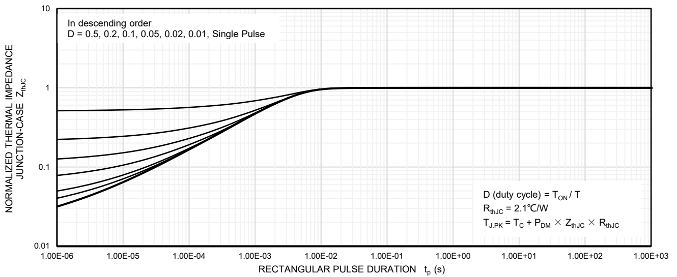
Transient Thermal Impedance, Junction-Case
