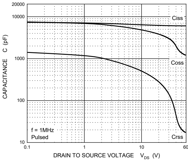
Typical Capacitances
