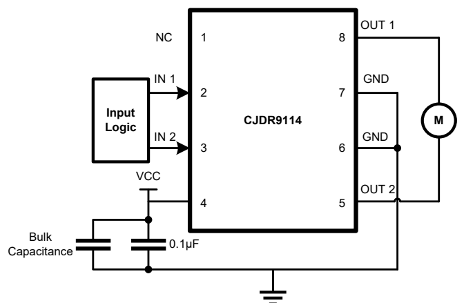
Figure 4-1. Typical Application Circuits
