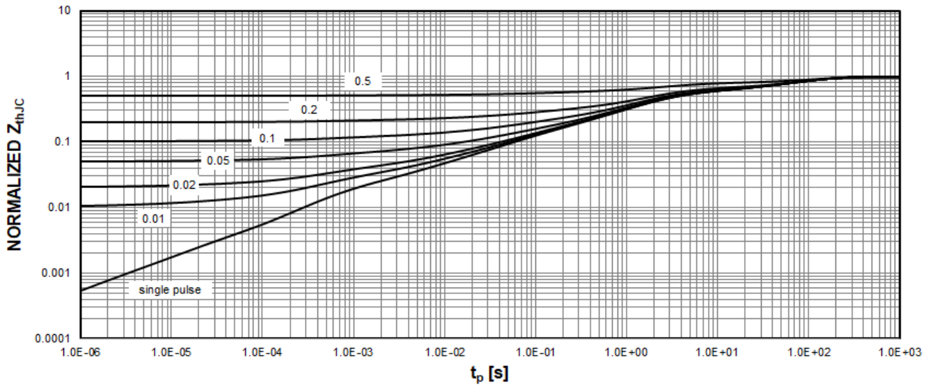
Transient Thermal Impedance, Junction-Ambient
