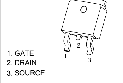
TO-252-2L
