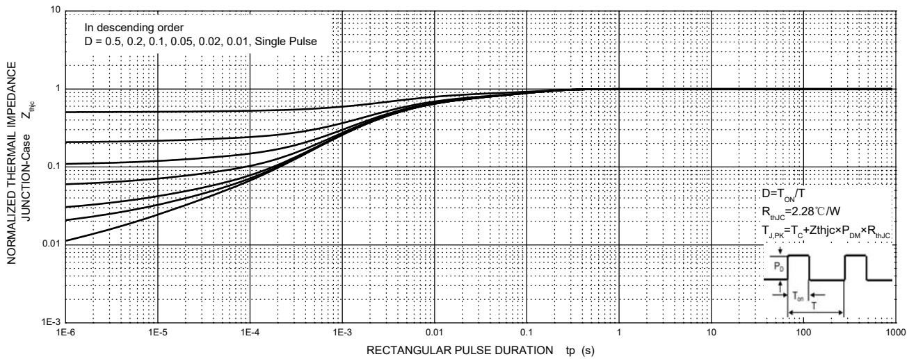
CSD06H65 Transient Thermal Impedance, Junction-Case
