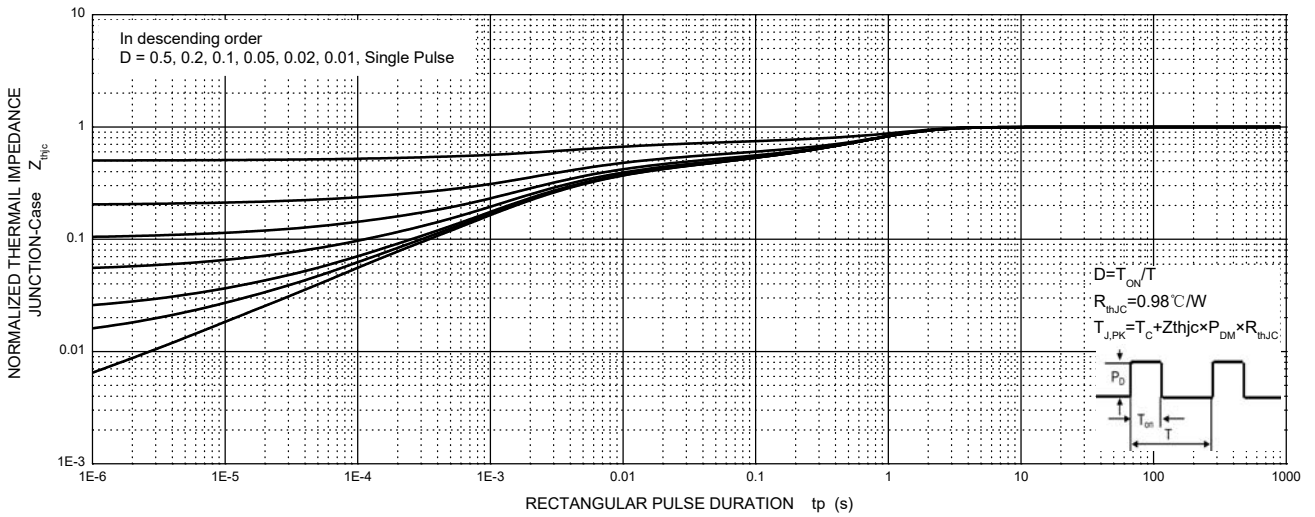
CSDW20H65 Transient Thermal Impedance, Junction-Case
