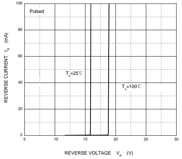
Reverse Characteristics
