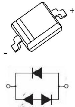
SOD-323
