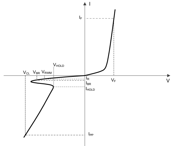
V-I characteristics for a Uni-direction TVS
