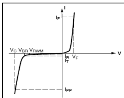
V-I characteristics for a Uni-direction ESD Protection Diode
