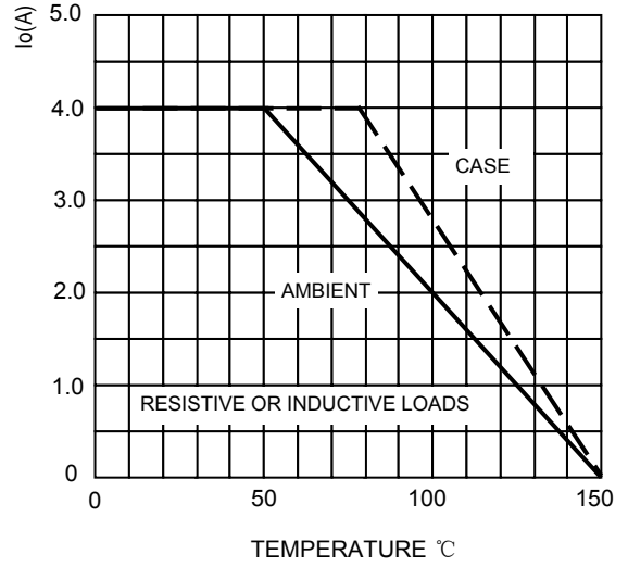
FIG.2-FORWARD DERATING CURRENT
