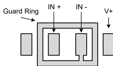
Figure 9-4. Guard Ring
