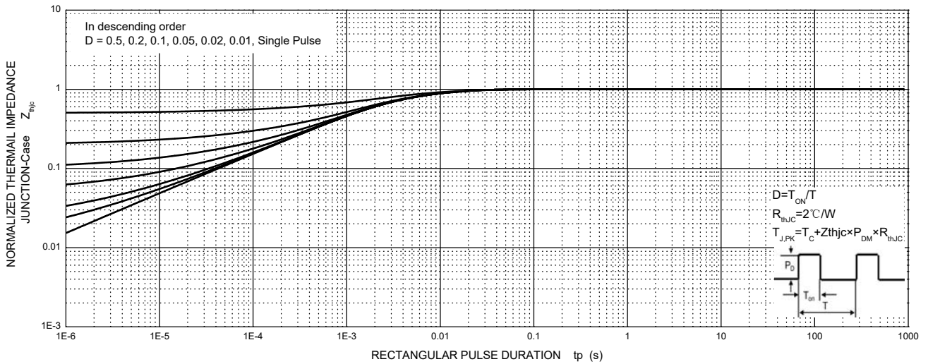
MUR1040CT Transient Thermal Impedance, Junction-Case
