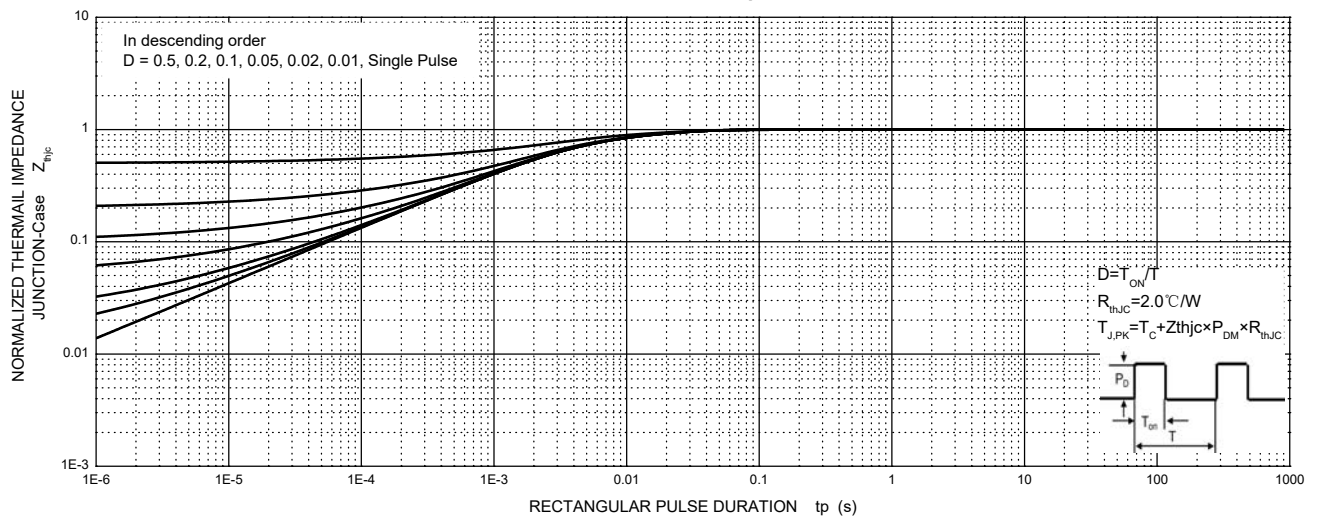
MUR1060CT Transient Thermal Impedance, Junction-Case
