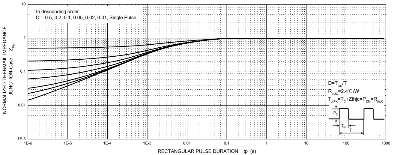
MUR10H60 Transient Thermal Impedance, Junction-Case
