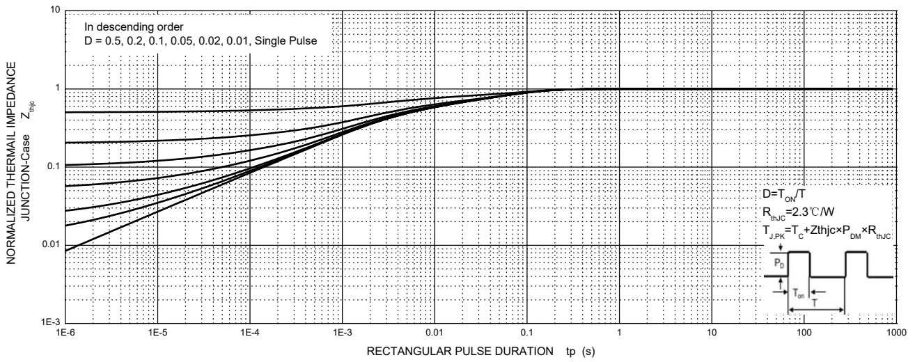
MUR15H120 Transient Thermal Impedance, Junction-Case
