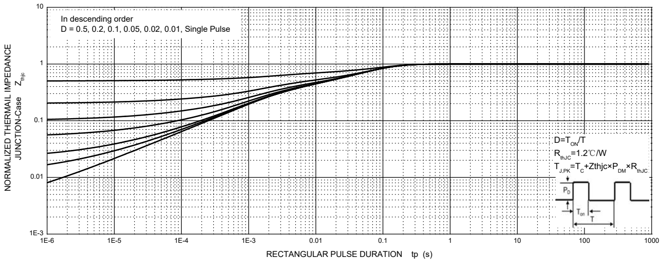
MUR30H60 Transient Thermal Impedance, Junction-Case
