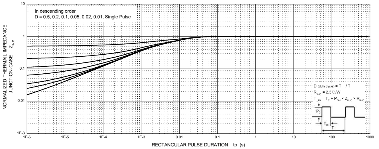
MURD10H120L Transient Thermal Impedance, Junction-Case
