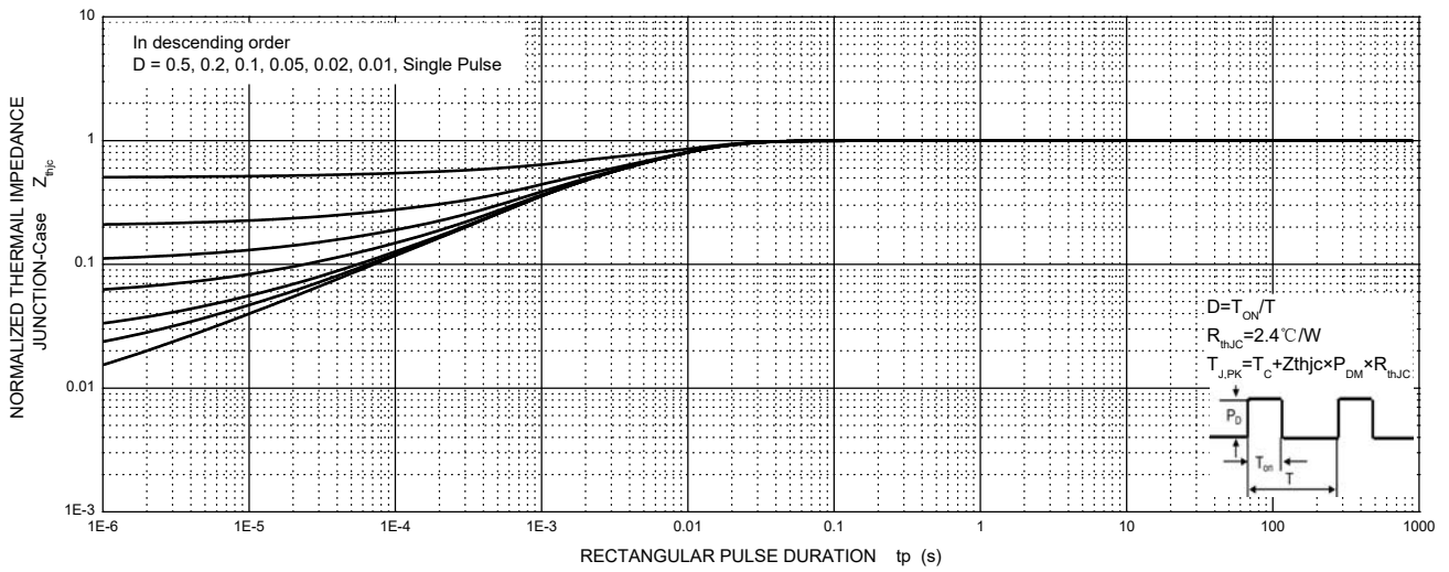
MURD10H30A Transient Thermal Impedance, Junction-Case
