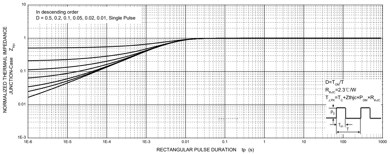
MURD10H60 Transient Thermal Impedance, Junction-Case
