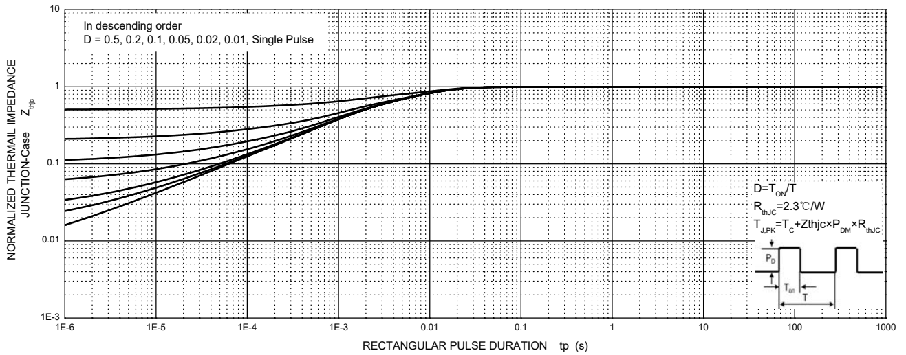
MURD10HS60 Transient Thermal Impedance, Junction-Case
