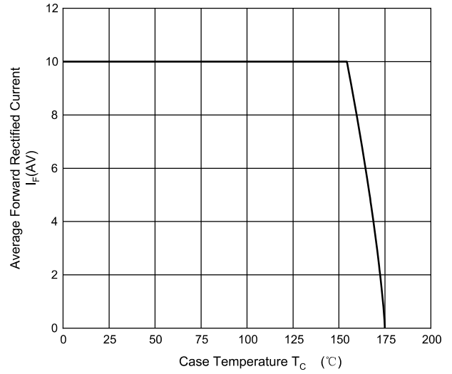
Current Derating
