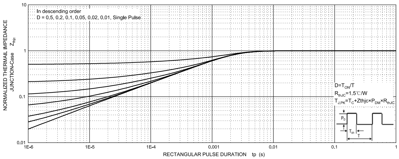
MURD10HS65 Transient Thermal Impedance, Junction-Case
