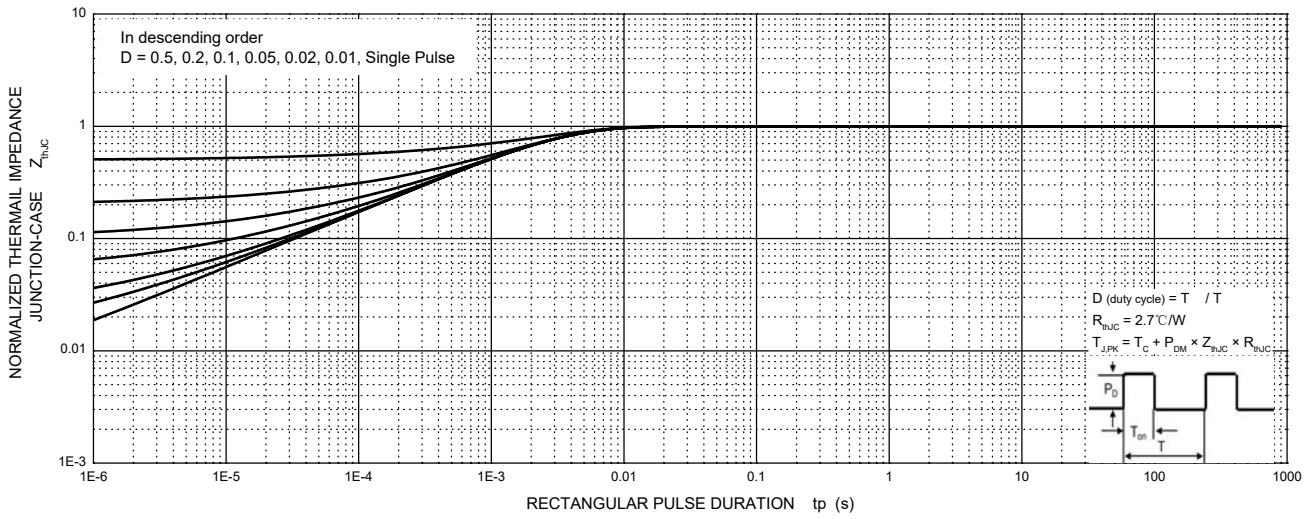
MURD16H20CT Transient Thermal Impedance, Junction-Case
