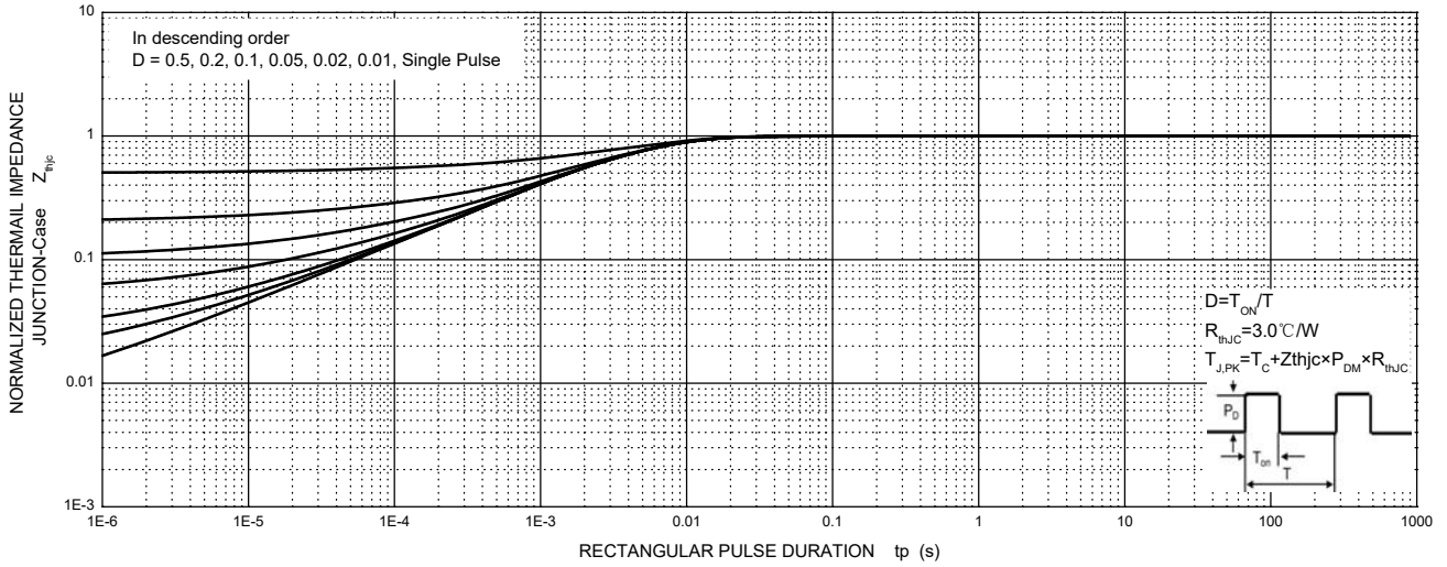
MURD8H60 Transient Thermal Impedance, Junction-Case
